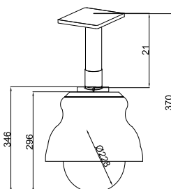
External Dimensions
