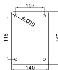
External Dimensions
