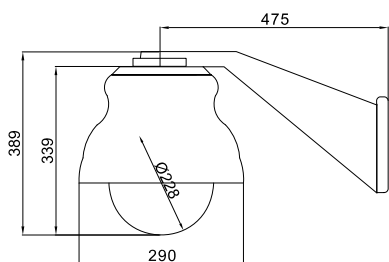
External Dimensions
